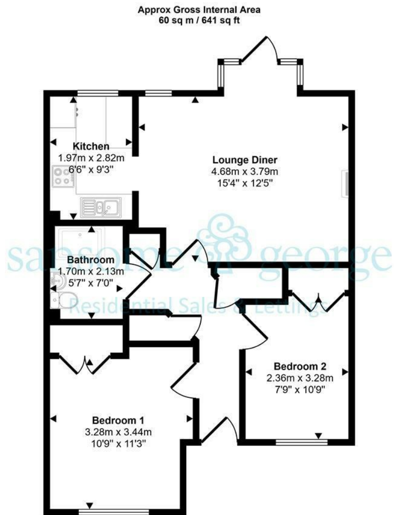
Floorplan
